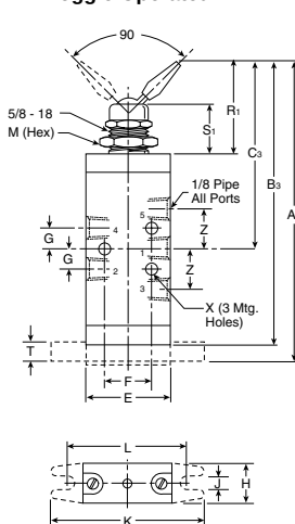
Toggle Operated
