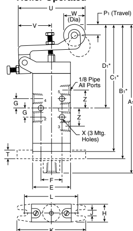
Roller Operated
