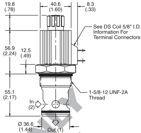
Normally Open
