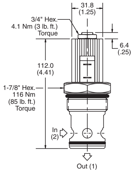
Normally Closed
